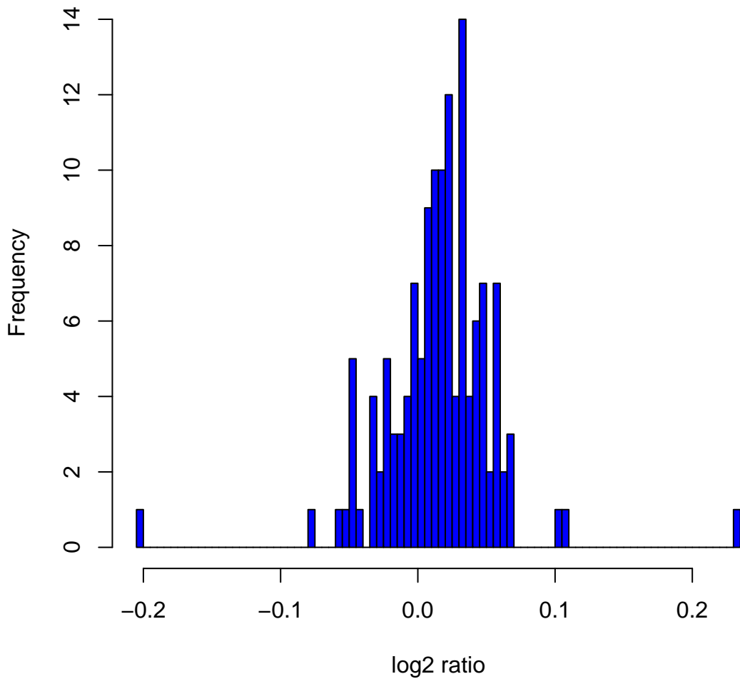
Histogram of log2ratios in 142 HapMap male samples at clone ChrXtp-3D8
