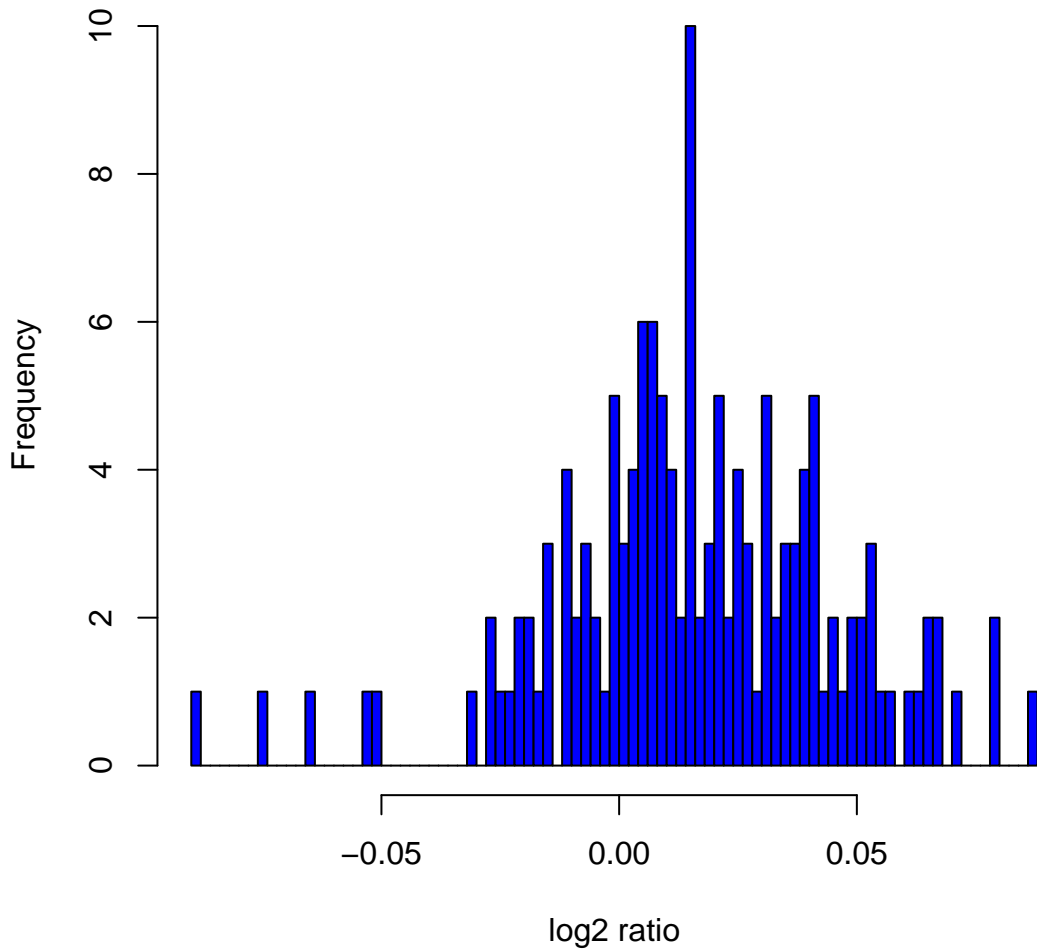
Histogram of log 2 ratios in 142 HapMap male samples at clone ChrXtp-5C11
