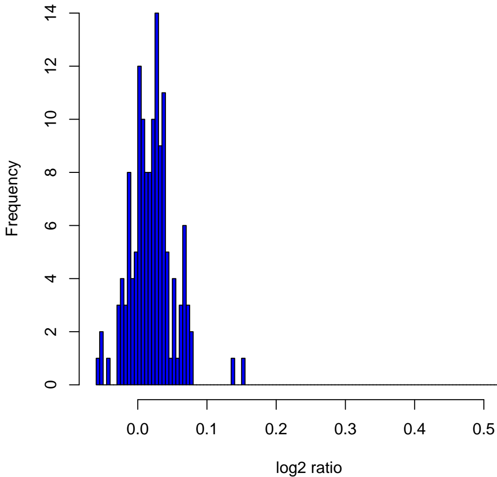
Histogram of log 2 ratios in 142 HapMap male samples at clone ChrXtp-5E11
