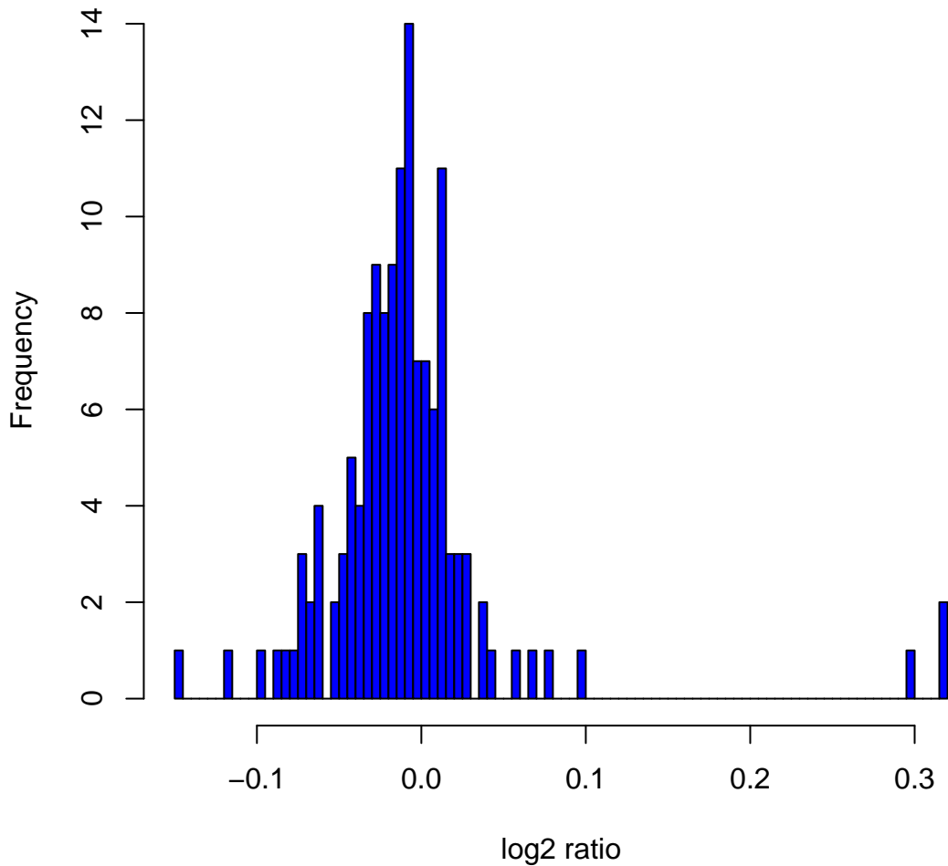
Histogram of log 2 ratios in 142 HapMap male samples at clone ChrXtp-5G10
