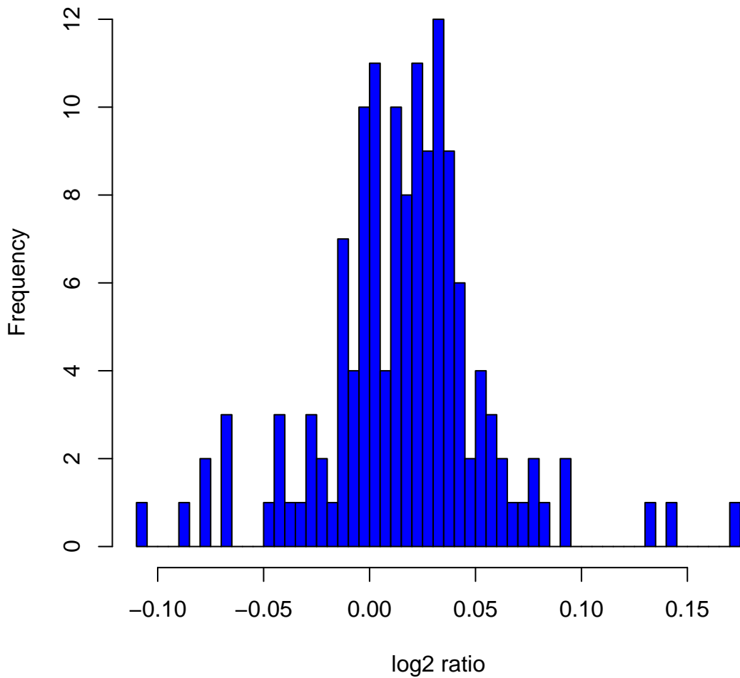
Histogram of log2ratios in 142 HapMap male samples at clone ChrXtp-5G9
