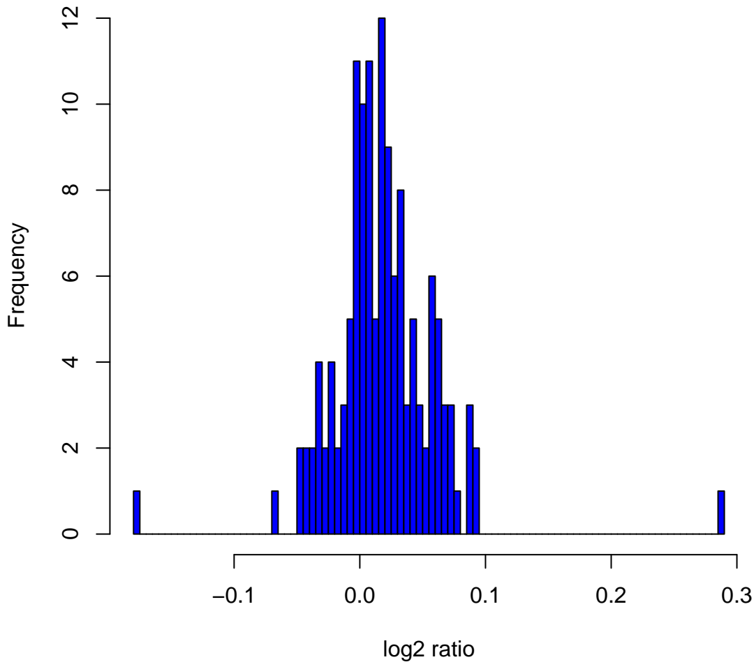
Histogram of log 2 ratios in 142 HapMap male samples at clone ChrXtp-6B10
