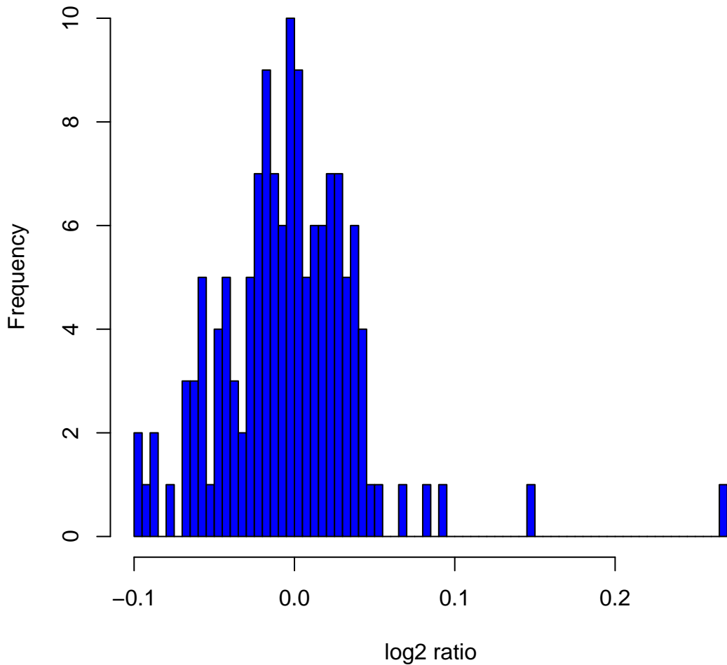
Histogram of \log_2 ratios in 142 HapMap male samples at clone ChrXtp-7B12
