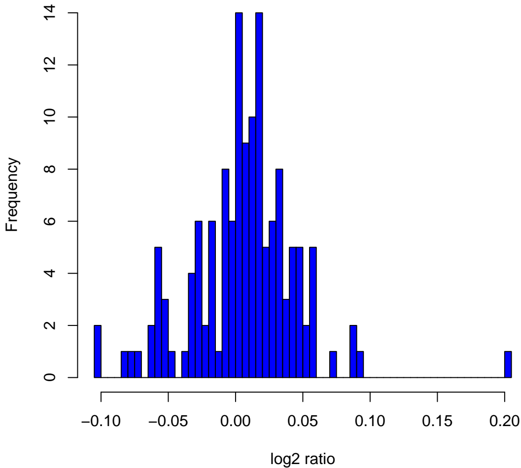
Histogram of log2ratios in 142 HapMap male samples at clone ChrXtp-7F3
