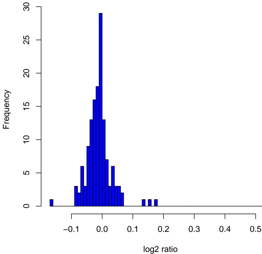
Histogram of \log_2 ratios in 142 HapMap male samples at clone ChrXtp-7G10
