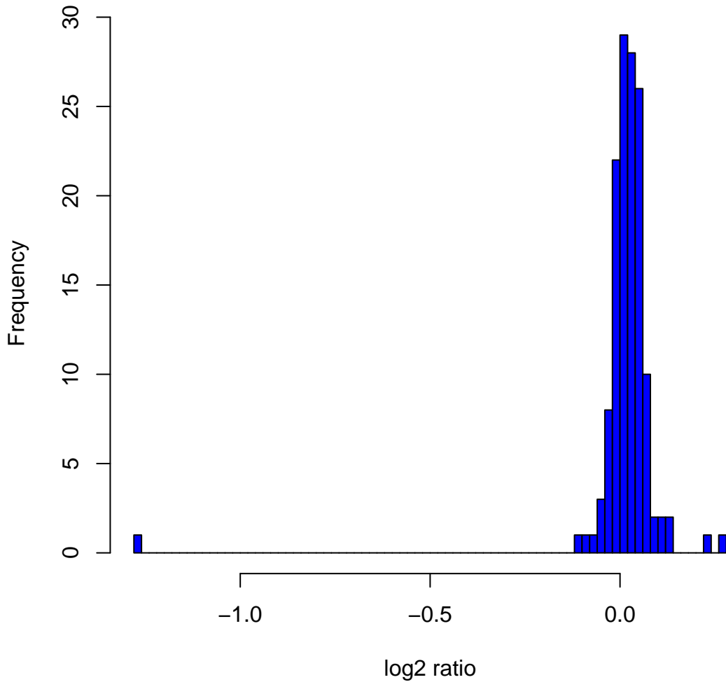
Histogram of log2ratios in 142 HapMap male samples at clone ChrXtp-8C2
