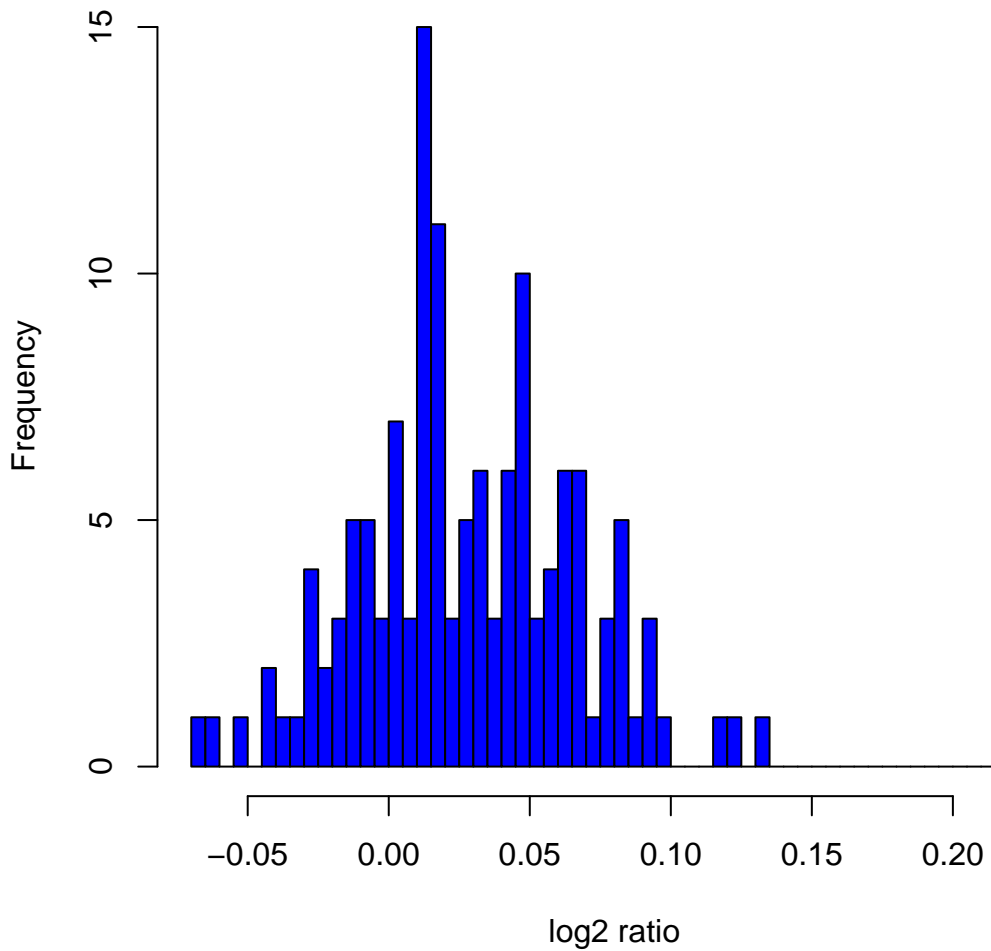
Histogram of log2ratios in 142 HapMap male samples at clone ChrXtp-9C3
