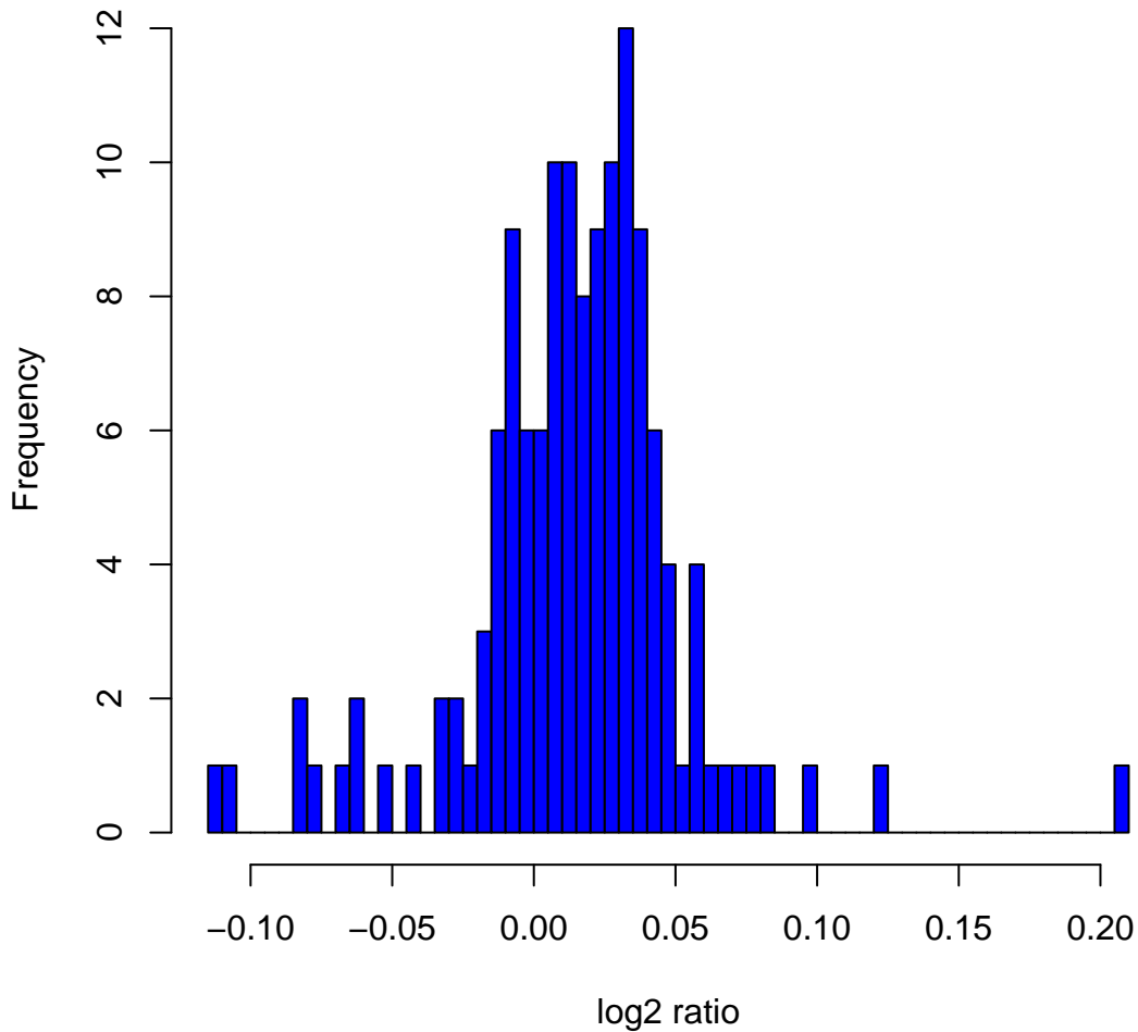
Histogram of log 2 ratios in 142 HapMap male samples at clone ChrXtp-9F11
