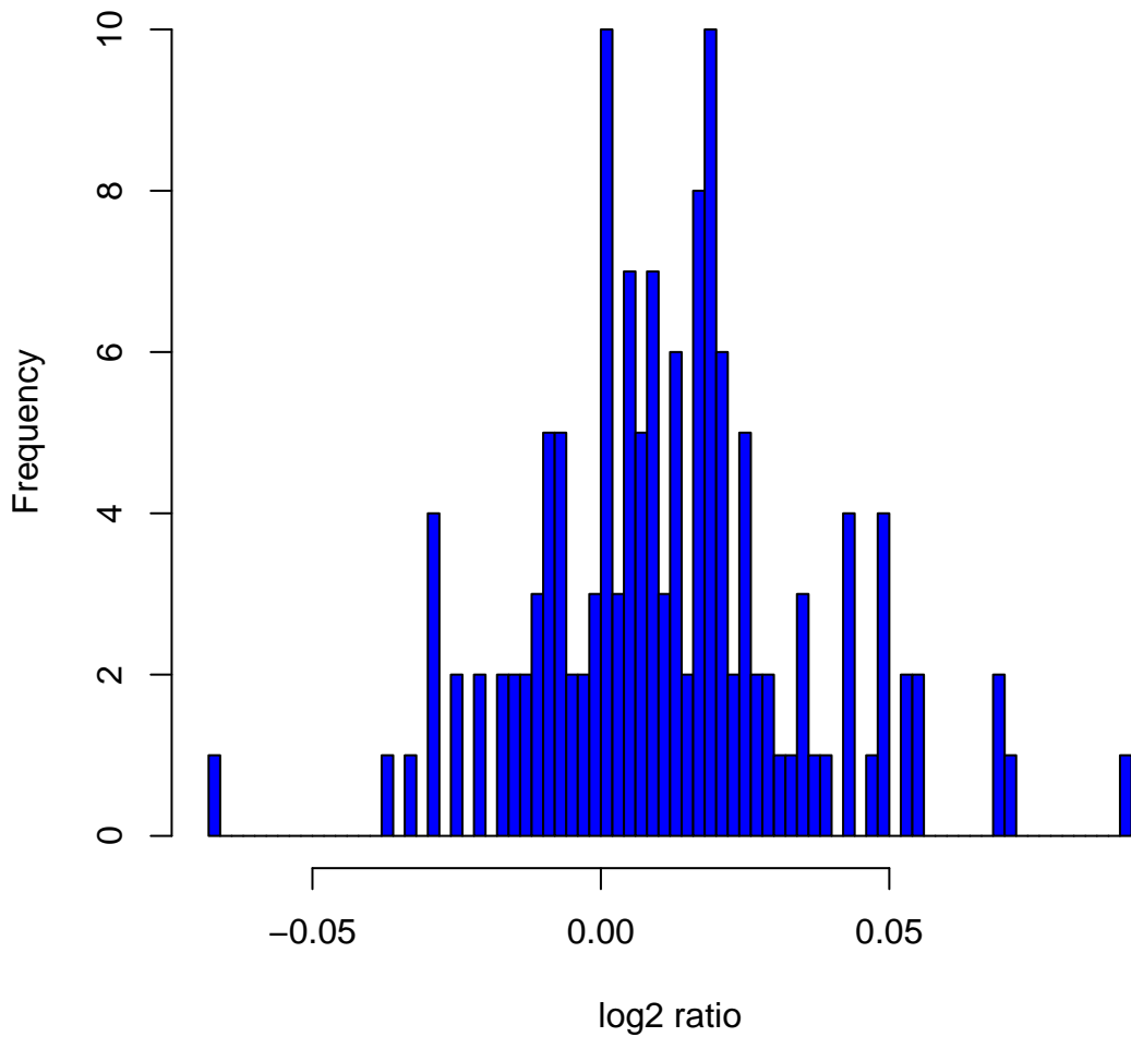
Histogram of log2ratios in 142 HapMap male samples at clone ChrYtp-1B2
