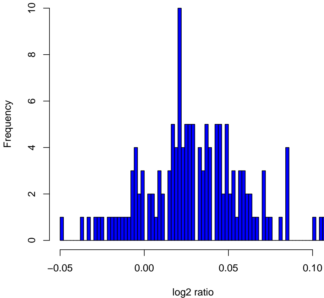
Histogram of \log_2 ratios in 142 HapMap male samples at clone ChrYtp-1E10
