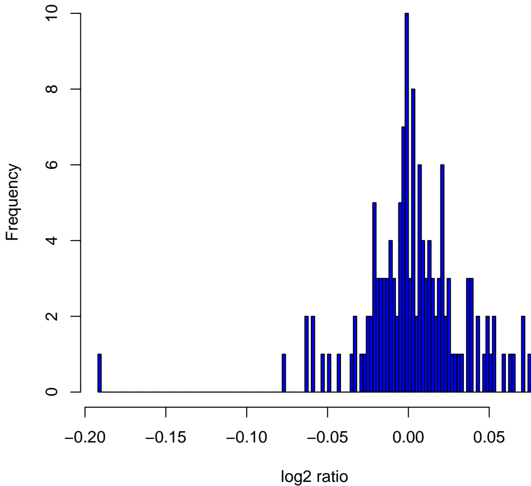
Histogram of log 2 ratios in 142 HapMap male samples at clone ChrYtp-1F11
