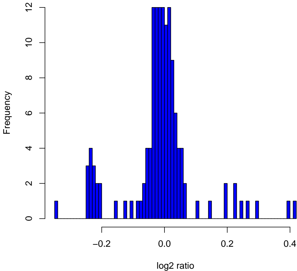
Histogram of log2ratios in 142 HapMap male samples at clone ChrYtp-2G5
