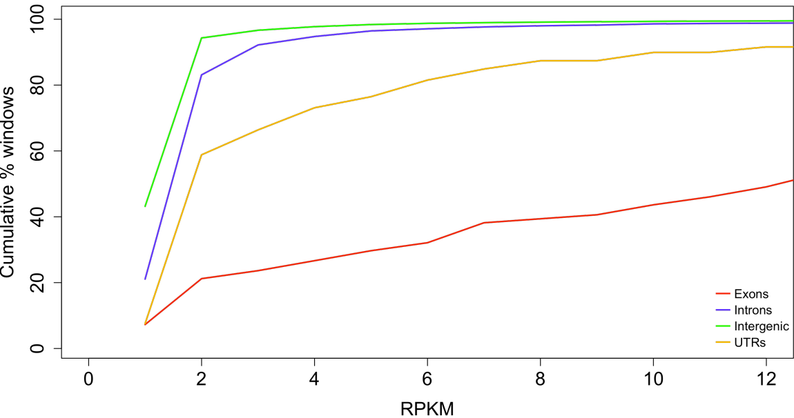
Estimation of the minimum RPKM value to discriminate between signal and noise
