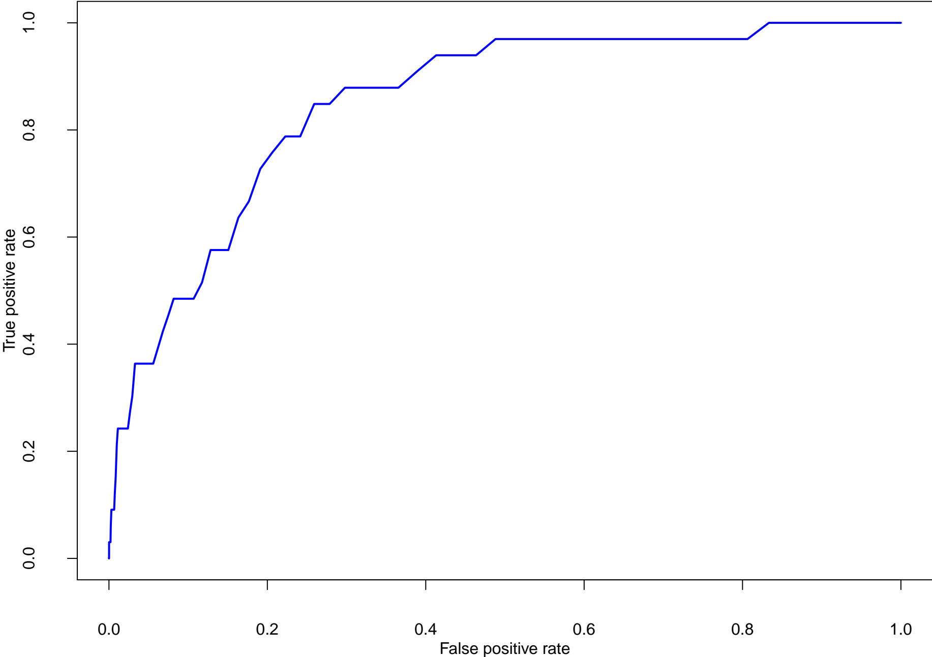
Classification results for HGMD spike-ins in NA06984 (AUC = 0.85)
