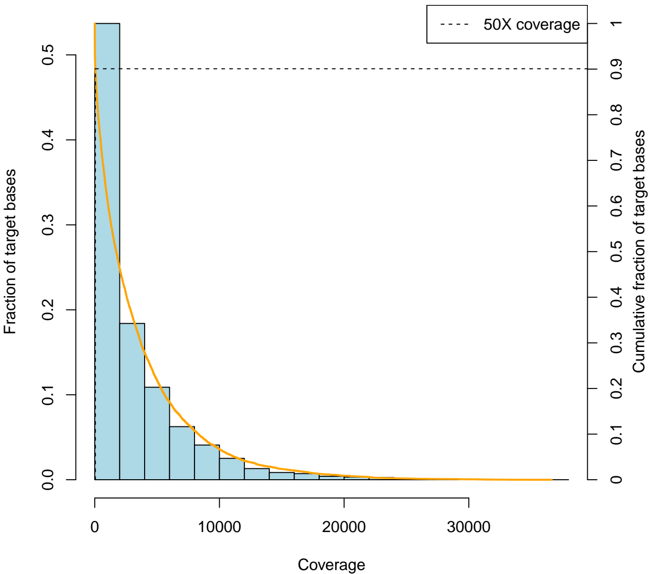
8016_7_9_hist_coverage
