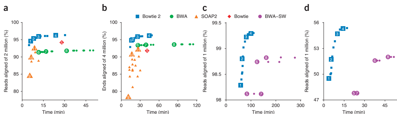
Figure 1 | Alignment comparison using HiSeq 2000, 454 and Ion Torrent reads. (a–d) Bowtie 2, BWA, SOAP2 and Bowtie were used to align two million 100 nt \times 100 nt paired-end HiSeq 2000 reads from a resequencing study 11 . Shown are results for unpaired alignment of end 1 (a), paired-end alignment (b), Bowtie 2 and BWA-SW alignment of 1 million 454 reads from the 1000 Genomes Project Pilot 12 (c), and Bowtie 2 and BWA-SW to align one million Ion Torrent reads from the G. Moore resequencing project 13 (d). Plotted is the percentage of reads for which at least one alignment was found. Each numbered point is data obtained using command-line parameters shown in Supplementary Table 1 .
