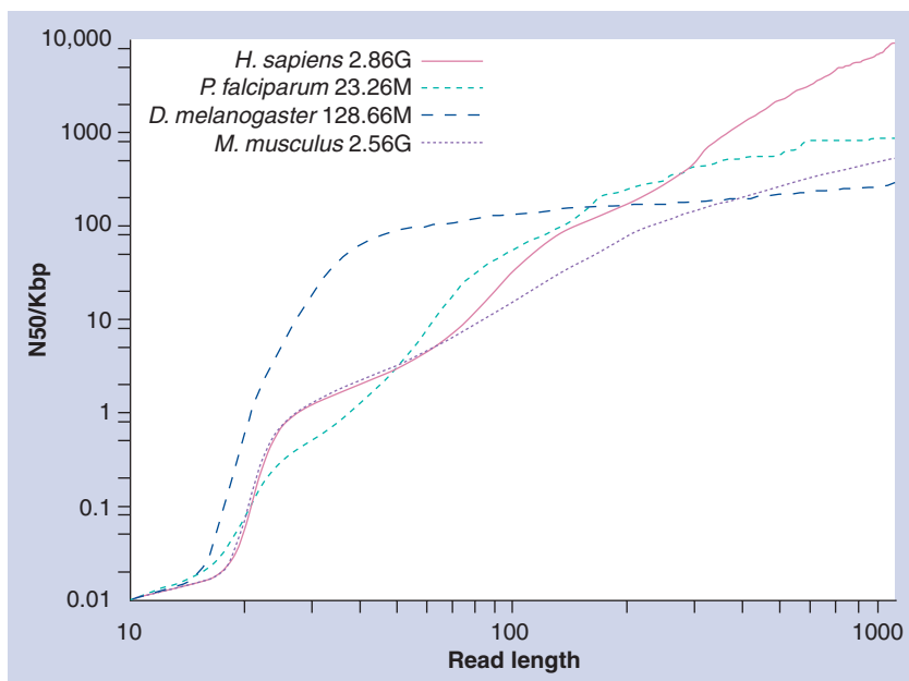
Figure 1. An upper bound on assembly N50 against read length y . For a set of sequences, the N50 is the number of bases in the longest sequence such that 50% of the total bases are contained in this sequence or longer sequences. Here, the N50 is given for the set of contiguous sequences of bases in each genome that are covered by a unique segment of sequence at a given length y . Owing to the ambiguities in ordering caused by nonunique sequences, this provides an upper bound on the N50 that is possible for whole-genome sequencing assembly when using reads below this length, and gives an indication of the advantages to be gained from longer read length in some cases.
